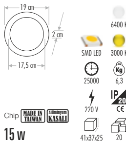
CT-5149 8" PANEL LED ARMATÜR
